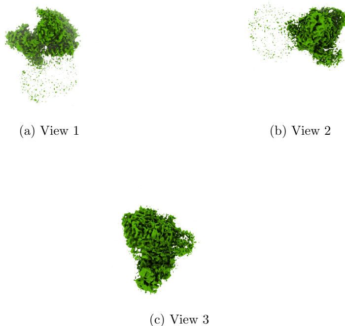
Figure 4: Isosurface at threshold=0.065000. Views generated by ChimeraX at a the following X, Y, Z angles: View 1 (0, -90, -90), View 2 (-90, 0, -90), View 3 (0, 0, 0).
