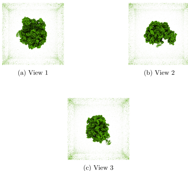
Figure 4: Isosurface at threshold=0.004340. Views generated by ChimeraX at a the following X, Y, Z angles: View 1 (0, -90, -90), View 2 (-90, 0, -90), View 3 (0, 0, 0).
