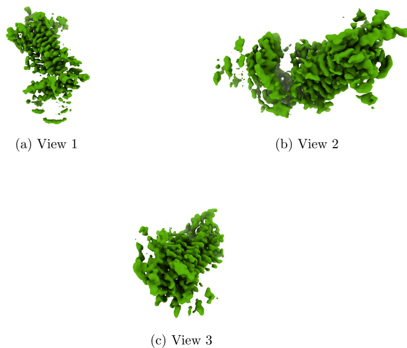
Figure 4: Isosurface at threshold=0.085300. Views generated by ChimeraX at a the following X, Y, Z angles: View 1 (0, -90, -90), View 2 (-90, 0, -90), View 3 (0, 0, 0).
