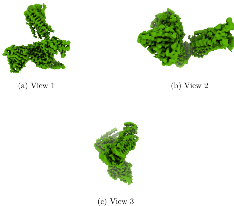
Figure 4: Isosurface at threshold=0.060300. Views generated by ChimeraX at a the following X, Y, Z angles: View 1 (0, -90, -90), View 2 (-90, 0, -90), View 3 (0, 0, 0).
