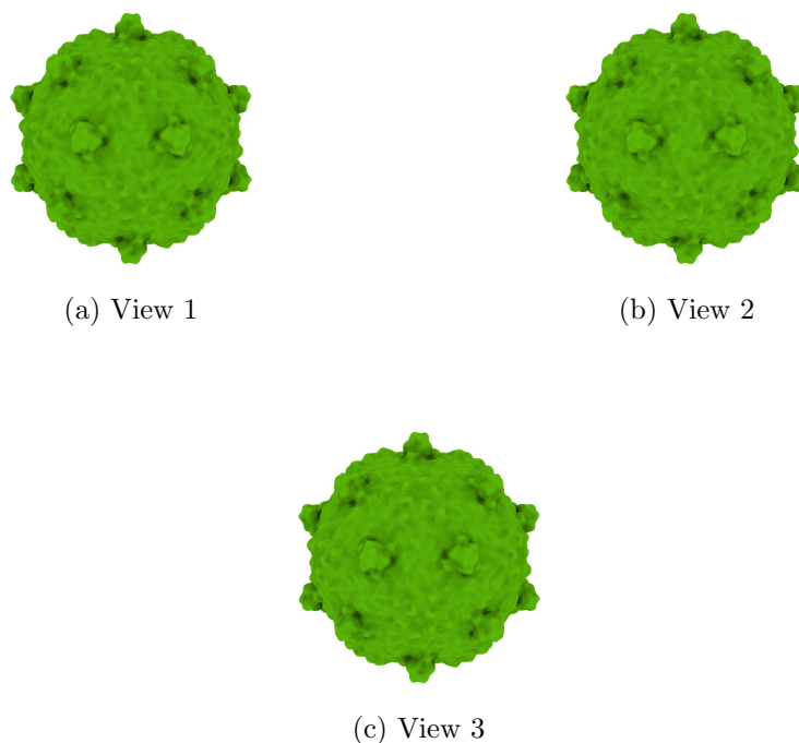
Figure 4: Isosurface at threshold=0.054300. Views generated by ChimeraX at a the following X, Y, Z angles: View 1 (0, -90, -90), View 2 (-90, 0, -90), View 3 (0, 0, 0).
