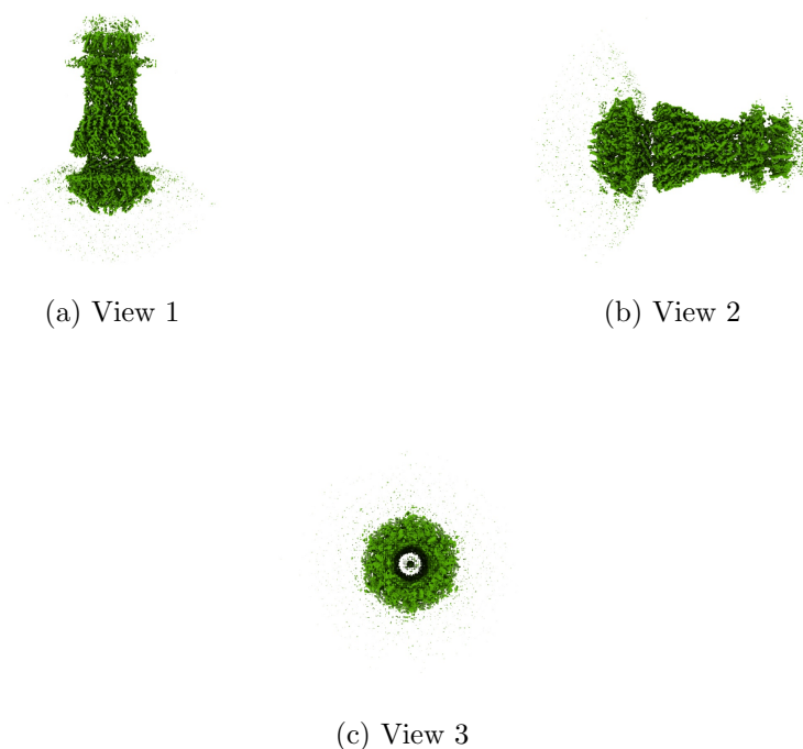
Figure 4: Isosurface at threshold=0.555000. Views generated by ChimeraX at a the following X, Y, Z angles: View 1 (0, -90, -90), View 2 (-90, 0, -90), View 3 (0, 0, 0).
