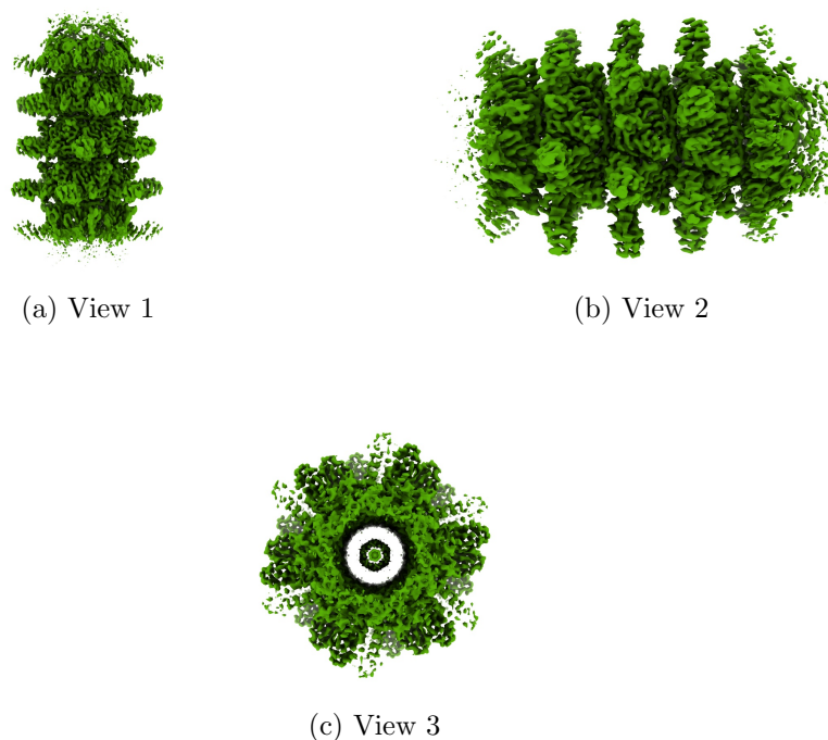
Figure 4: Isosurface at threshold=0.453000. Views generated by ChimeraX at a the following X, Y, Z angles: View 1 (0, -90, -90), View 2 (-90, 0, -90), View 3 (0, 0, 0).
