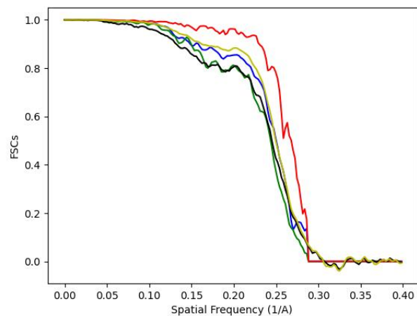
Figure 36: FSC in X, Y, Z, the global FSC, and the Average Cosine Phase.
