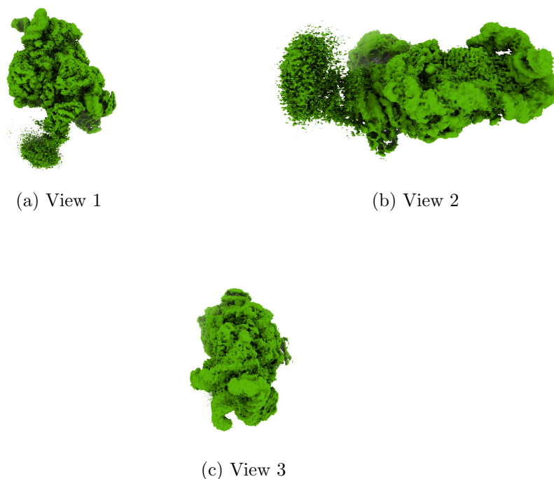
Figure 4: Isosurface at threshold=0.092600. Views generated by ChimeraX at a the following X, Y, Z angles: View 1 (0, -90, -90), View 2 (-90, 0, -90), View 3 (0, 0, 0).
