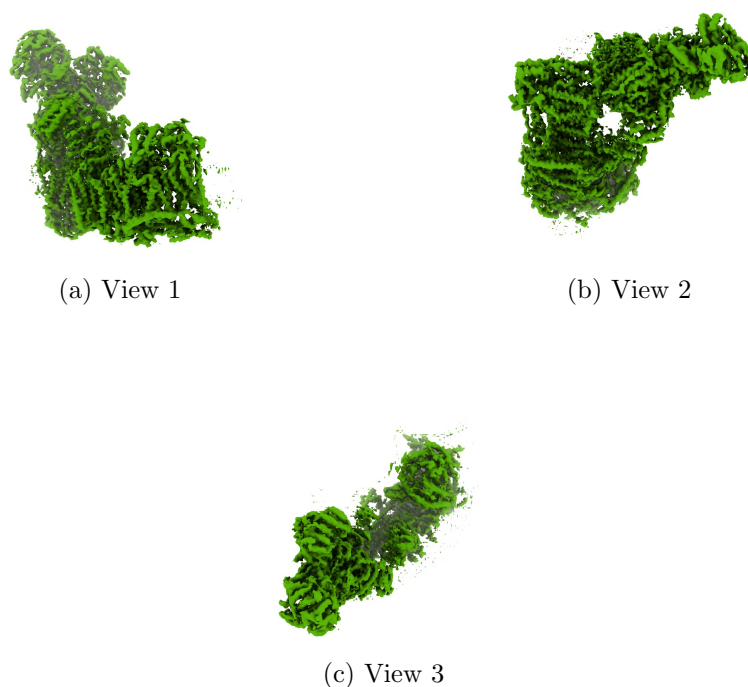
Figure 4: Isosurface at threshold=0.061500. Views generated by ChimeraX at a the following X, Y, Z angles: View 1 (0, -90, -90), View 2 (-90, 0, -90), View 3 (0, 0, 0).
