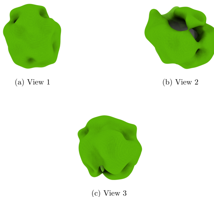
Figure 4: Isosurface at threshold=8.900000. Views generated by ChimeraX at a the following X, Y, Z angles: View 1 (0, -90, -90), View 2 (-90, 0, -90), View 3 (0, 0, 0).
