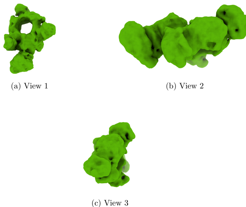
Figure 4: Isosurface at threshold=0.059000. Views generated by ChimeraX at a the following X, Y, Z angles: View 1 (0, -90, -90), View 2 (-90, 0, -90), View 3 (0, 0, 0).
