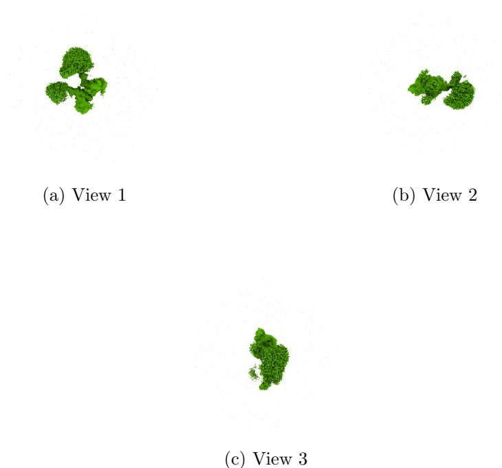
Figure 4: Isosurface at threshold=0.068900. Views generated by ChimeraX at a the following X, Y, Z angles: View 1 (0, -90, -90), View 2 (-90, 0, -90), View 3 (0, 0, 0).
