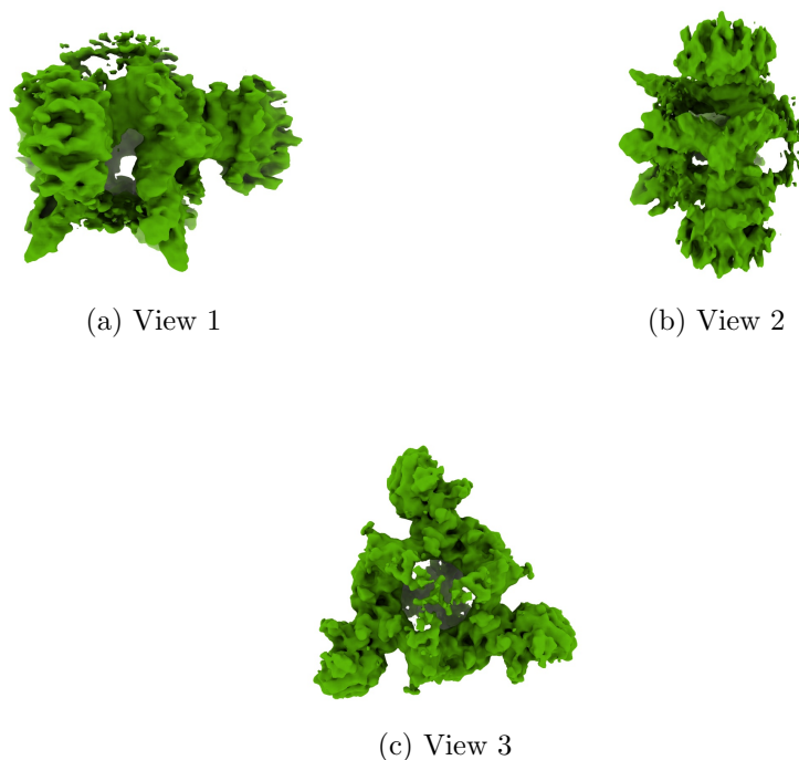
Figure 4: Isosurface at threshold=0.055900. Views generated by ChimeraX at a the following X, Y, Z angles: View 1 (0, -90, -90), View 2 (-90, 0, -90), View 3 (0, 0, 0).
