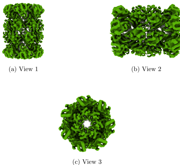
Figure 4: Isosurface at threshold=0.047100. Views generated by ChimeraX at a the following X, Y, Z angles: View 1 (0, -90, -90), View 2 (-90, 0, -90), View 3 (0, 0, 0).
