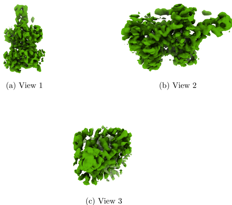
Figure 4: Isosurface at threshold=0.008000. Views generated by ChimeraX at a the following X, Y, Z angles: View 1 (0, -90, -90), View 2 (-90, 0, -90), View 3 (0, 0, 0).
