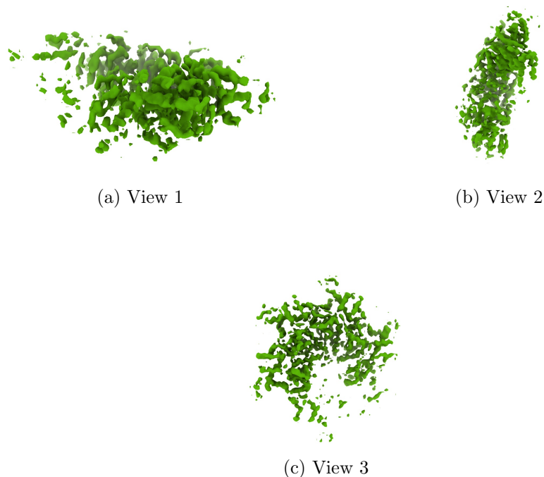
Figure 4: Isosurface at threshold=0.053900. Views generated by ChimeraX at a the following X, Y, Z angles: View 1 (0, -90, -90), View 2 (-90, 0, -90), View 3 (0, 0, 0).
