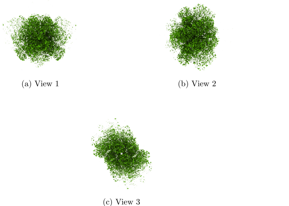
Figure 4: Isosurface at threshold=0.020000. Views generated by ChimeraX at a the following X, Y, Z angles: View 1 (0, -90, -90), View 2 (-90, 0, -90), View 3 (0, 0, 0).
