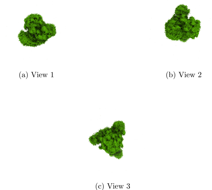
Figure 4: Isosurface at threshold=0.066800. Views generated by ChimeraX at a the following X, Y, Z angles: View 1 (0, -90, -90), View 2 (-90, 0, -90), View 3 (0, 0, 0).
