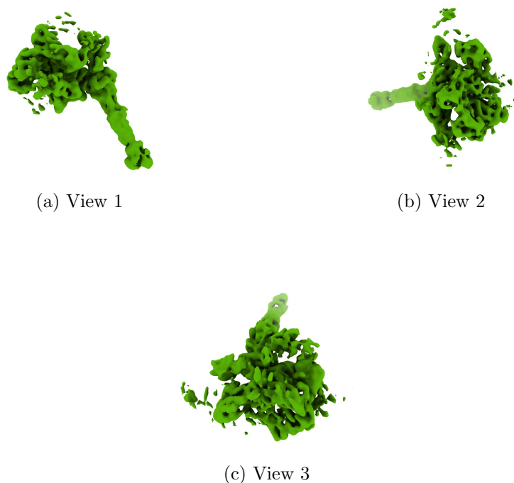
Figure 4: Isosurface at threshold=0.095000. Views generated by ChimeraX at a the following X, Y, Z angles: View 1 (0, -90, -90), View 2 (-90, 0, -90), View 3 (0, 0, 0).
