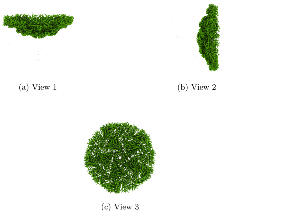
Figure 4: Isosurface at threshold=0.420000. Views generated by ChimeraX at a the following X, Y, Z angles: View 1 (0, -90, -90), View 2 (-90, 0, -90), View 3 (0, 0, 0).
