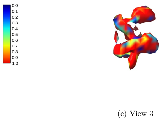
Figure 15: Local occupancy according to LocOccupancy. Views generated by ChimeraX at the following X, Y, Z angles: View 1 (0, -90, -90), View 2 (-90, 0, -90), View 3 (0, 0, 0).
