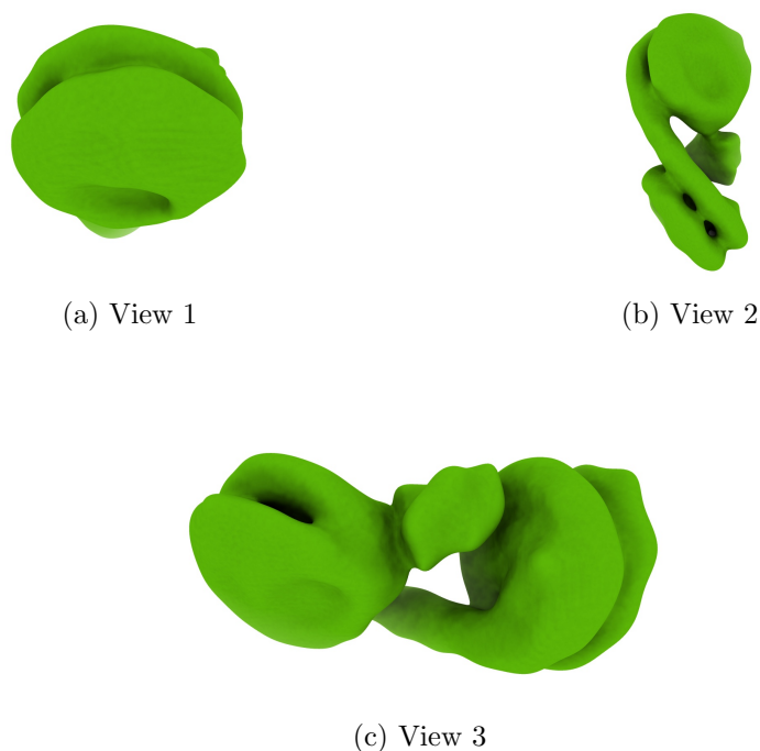
Figure 4: Isosurface at threshold=3.250000. Views generated by ChimeraX at a the following X, Y, Z angles: View 1 (0, -90, -90), View 2 (-90, 0, -90), View 3 (0, 0, 0).
