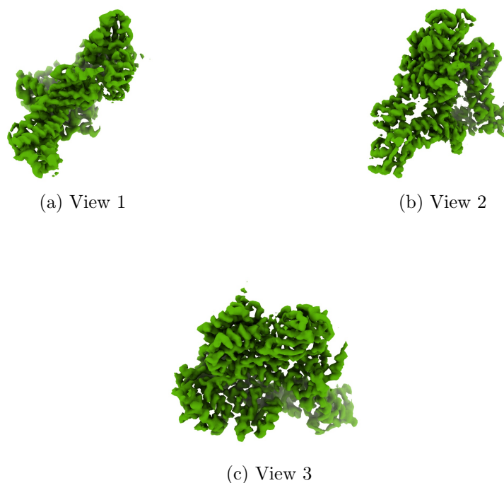
Figure 4: Isosurface at threshold=0.037000. Views generated by ChimeraX at a the following X, Y, Z angles: View 1 (0, -90, -90), View 2 (-90, 0, -90), View 3 (0, 0, 0).
