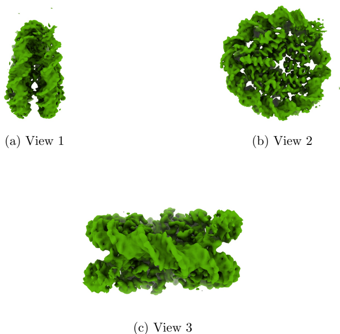
Figure 4: Isosurface at threshold=5.400000. Views generated by ChimeraX at a the following X, Y, Z angles: View 1 (0, -90, -90), View 2 (-90, 0, -90), View 3 (0, 0, 0).
