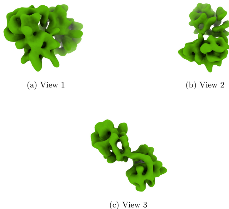
Figure 4: Isosurface at threshold=0.037800. Views generated by ChimeraX at a the following X, Y, Z angles: View 1 (0, -90, -90), View 2 (-90, 0, -90), View 3 (0, 0, 0).
