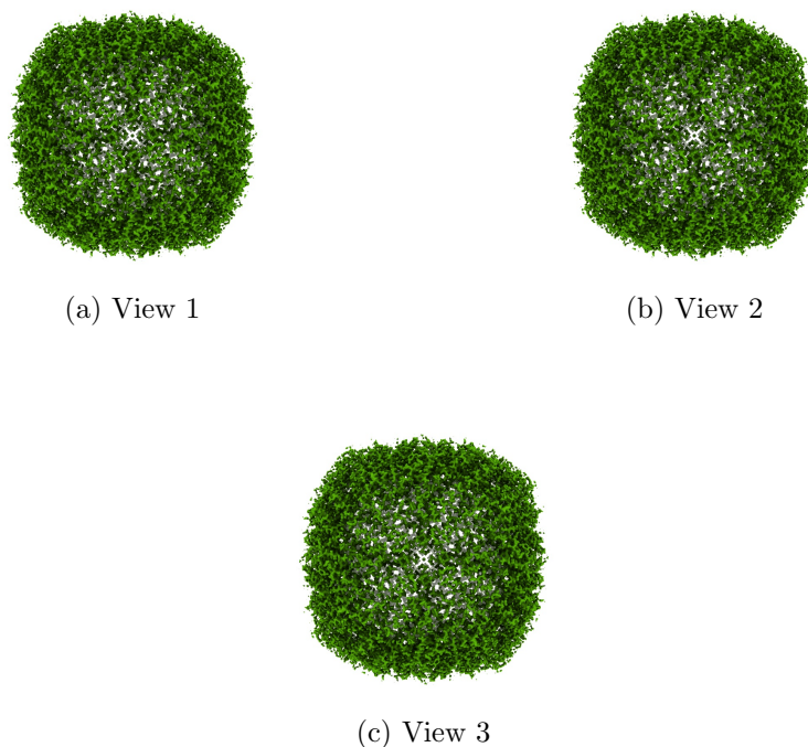
Figure 4: Isosurface at threshold=0.037900. Views generated by ChimeraX at a the following X, Y, Z angles: View 1 (0, -90, -90), View 2 (-90, 0, -90), View 3 (0, 0, 0).
