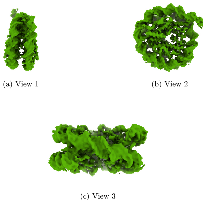
Figure 4: Isosurface at threshold=5.700000. Views generated by ChimeraX at a the following X, Y, Z angles: View 1 (0, -90, -90), View 2 (-90, 0, -90), View 3 (0, 0, 0).
