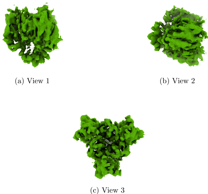
Figure 4: Isosurface at threshold=0.132000. Views generated by ChimeraX at a the following X, Y, Z angles: View 1 (0, -90, -90), View 2 (-90, 0, -90), View 3 (0, 0, 0).
