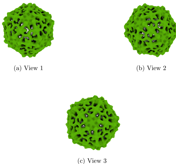
Figure 4: Isosurface at threshold=2.360000. Views generated by ChimeraX at a the following X, Y, Z angles: View 1 (0, -90, -90), View 2 (-90, 0, -90), View 3 (0, 0, 0).
