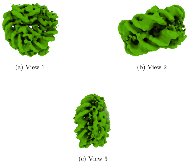
Figure 4: Isosurface at threshold=0.031600. Views generated by ChimeraX at a the following X, Y, Z angles: View 1 (0, -90, -90), View 2 (-90, 0, -90), View 3 (0, 0, 0).
