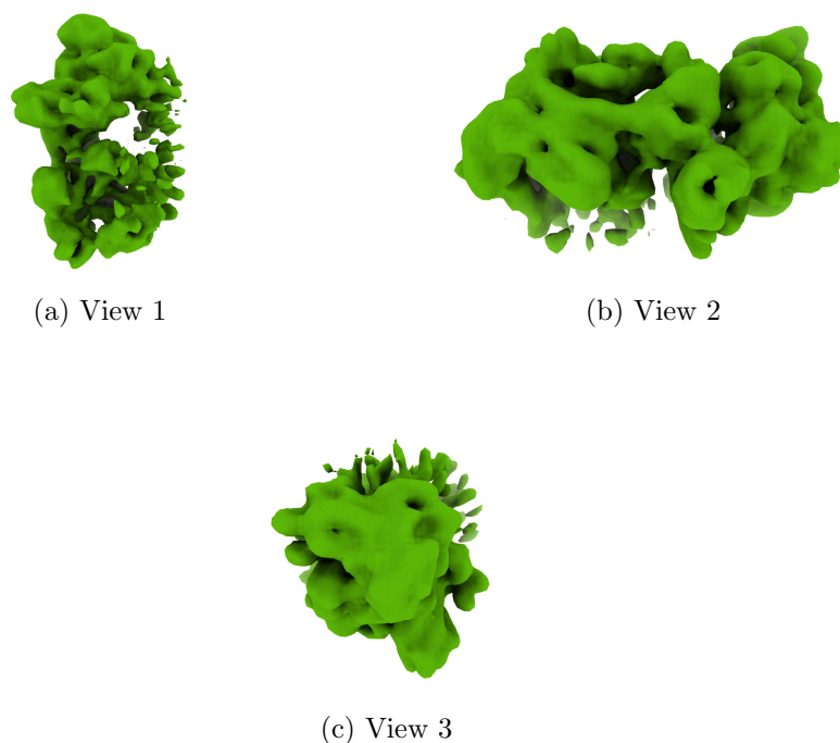
Figure 4: Isosurface at threshold=0.080000. Views generated by ChimeraX at the following X, Y, Z angles: View 1 (0, -90, -90), View 2 (-90, 0, -90), View 3 (0, 0, 0).
