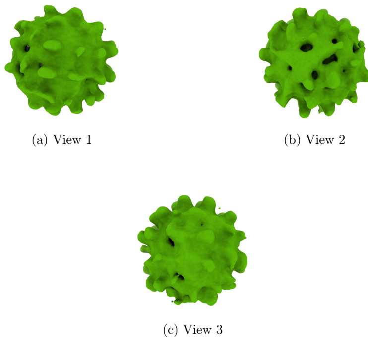
Figure 4: Isosurface at threshold=0.005970. Views generated by ChimeraX at a the following X, Y, Z angles: View 1 (0, -90, -90), View 2 (-90, 0, -90), View 3 (0, 0, 0).
