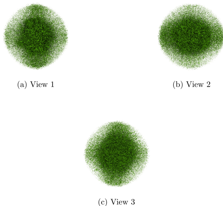
Figure 4: Isosurface at threshold=0.056300. Views generated by ChimeraX at a the following X, Y, Z angles: View 1 (0, -90, -90), View 2 (-90, 0, -90), View 3 (0, 0, 0).
