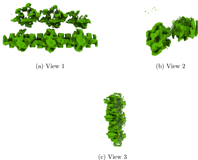
Figure 4: Isosurface at threshold=0.009000. Views generated by ChimeraX at a the following X, Y, Z angles: View 1 (0, -90, -90), View 2 (-90, 0, -90), View 3 (0, 0, 0).
