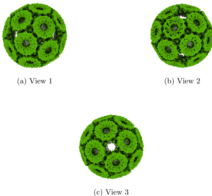
Figure 4: Isosurface at threshold=0.065000. Views generated by ChimeraX at the following X, Y, Z angles: View 1 (0, -90, -90), View 2 (-90, 0, -90), View 3 (0, 0, 0).
