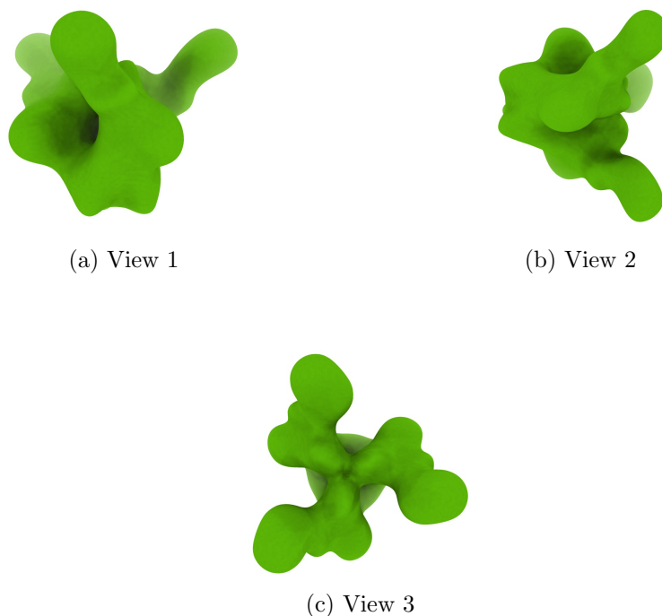
Figure 4: Isosurface at threshold=0.018800. Views generated by ChimeraX at a the following X, Y, Z angles: View 1 (0, -90, -90), View 2 (-90, 0, -90), View 3 (0, 0, 0).
