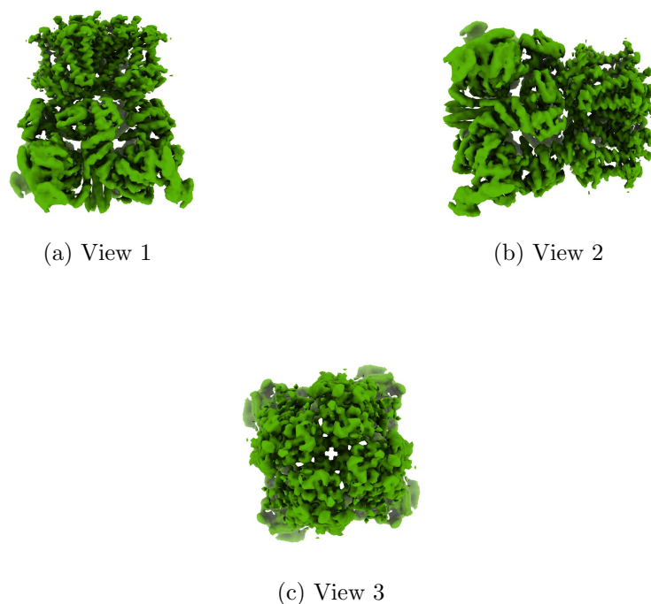
Figure 4: Isosurface at threshold=1.740000. Views generated by ChimeraX at a the following X, Y, Z angles: View 1 (0, -90, -90), View 2 (-90, 0, -90), View 3 (0, 0, 0).
