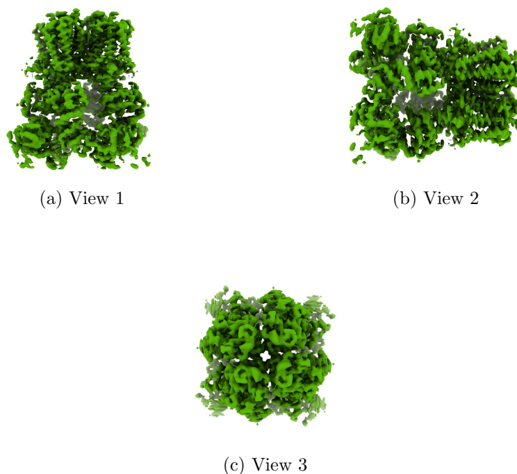
Figure 4: Isosurface at threshold=0.027800. Views generated by ChimeraX at a the following X, Y, Z angles: View 1 (0, -90, -90), View 2 (-90, 0, -90), View 3 (0, 0, 0).
