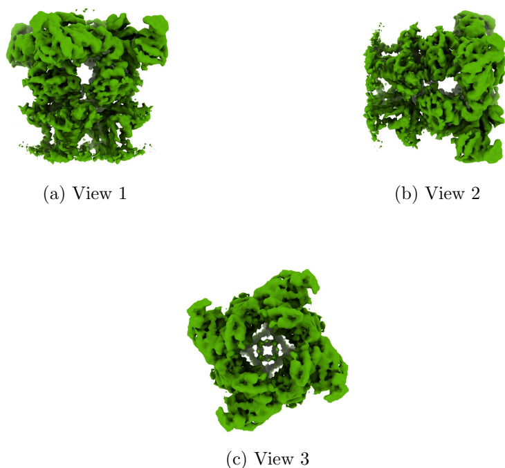
Figure 4: Isosurface at threshold=0.083300. Views generated by ChimeraX at a the following X, Y, Z angles: View 1 (0, -90, -90), View 2 (-90, 0, -90), View 3 (0, 0, 0).
