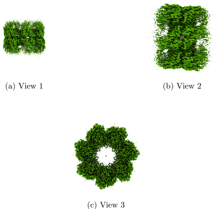
Figure 4: Isosurface at threshold=0.048300. Views generated by ChimeraX at a the following X, Y, Z angles: View 1 (0, -90, -90), View 2 (-90, 0, -90), View 3 (0, 0, 0).
