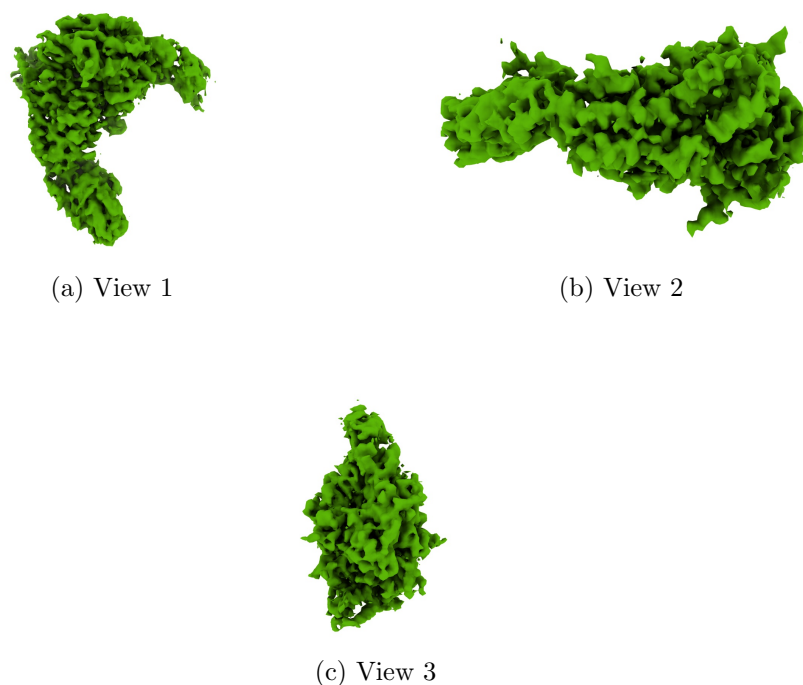
Figure 4: Isosurface at threshold=0.034900. Views generated by ChimeraX at a the following X, Y, Z angles: View 1 (0, -90, -90), View 2 (-90, 0, -90), View 3 (0, 0, 0).
