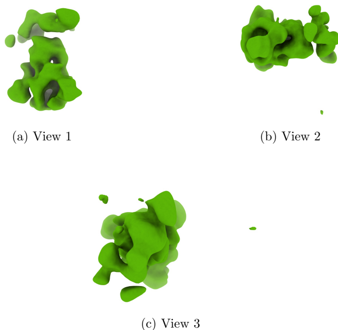
Figure 4: Isosurface at threshold=0.012300. Views generated by ChimeraX at a the following X, Y, Z angles: View 1 (0, -90, -90), View 2 (-90, 0, -90), View 3 (0, 0, 0).
