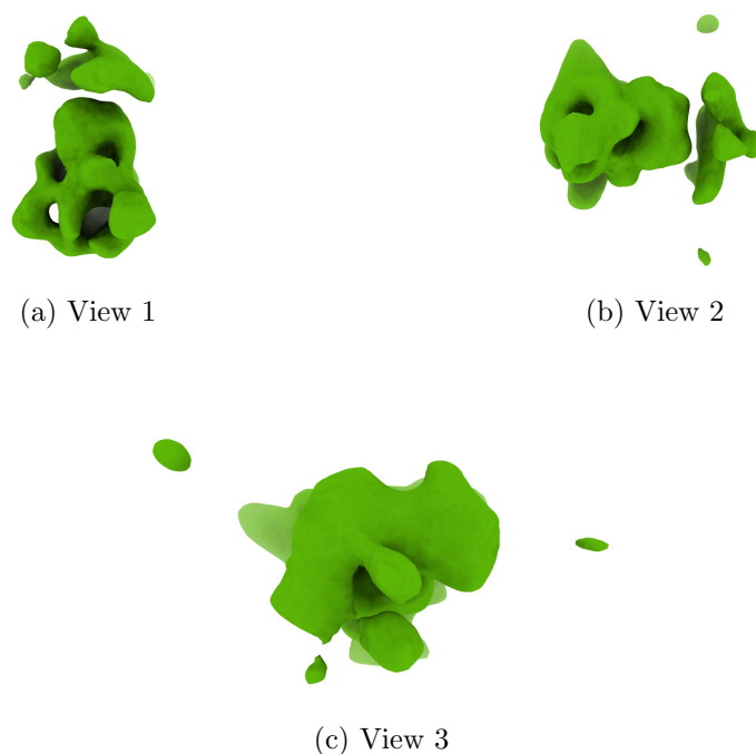
Figure 4: Isosurface at threshold=0.014000. Views generated by ChimeraX at a the following X, Y, Z angles: View 1 (0, -90, -90), View 2 (-90, 0, -90), View 3 (0, 0, 0).
