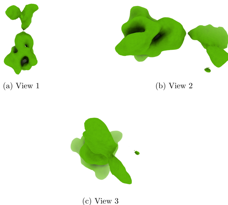
Figure 4: Isosurface at threshold=0.010700. Views generated by ChimeraX at a the following X, Y, Z angles: View 1 (0, -90, -90), View 2 (-90, 0, -90), View 3 (0, 0, 0).
