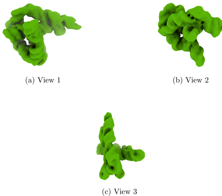
Figure 4: Isosurface at threshold=0.256000. Views generated by ChimeraX at a the following X, Y, Z angles: View 1 (0, -90, -90), View 2 (-90, 0, -90), View 3 (0, 0, 0).
