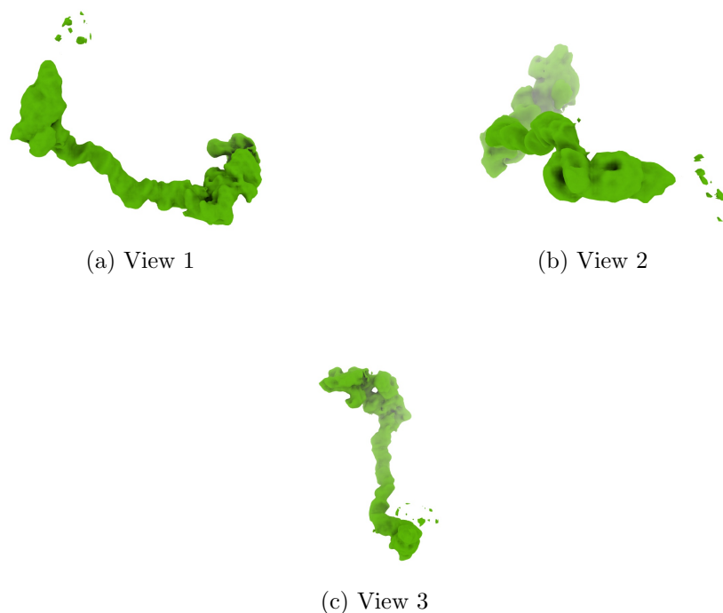
Figure 4: Isosurface at threshold=3.000000. Views generated by ChimeraX at a the following X, Y, Z angles: View 1 (0, -90, -90), View 2 (-90, 0, -90), View 3 (0, 0, 0).
