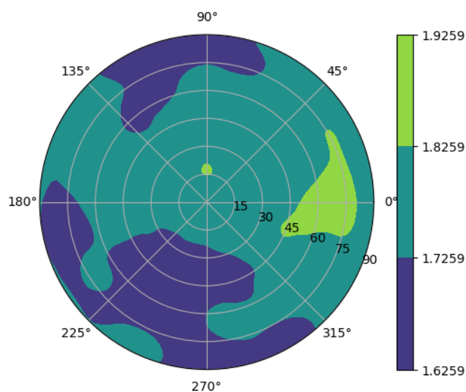
Figure 25: Directional resolution in the projection sphere.
