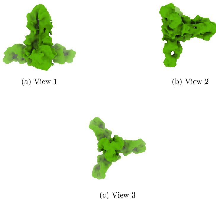
Figure 4: Isosurface at threshold=0.045200. Views generated by ChimeraX at a the following X, Y, Z angles: View 1 (0, -90, -90), View 2 (-90, 0, -90), View 3 (0, 0, 0).
