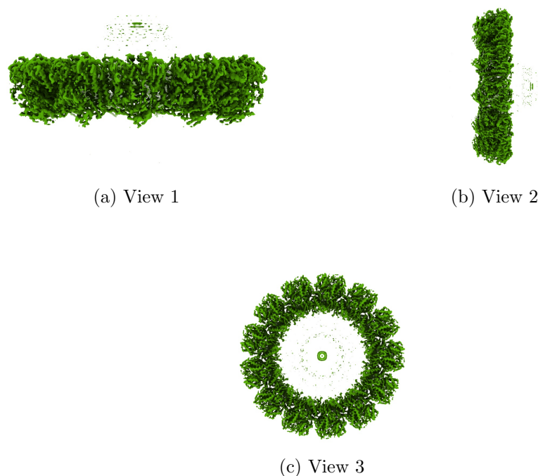
Figure 4: Isosurface at threshold=0.240000. Views generated by ChimeraX at a the following X, Y, Z angles: View 1 (0, -90, -90), View 2 (-90, 0, -90), View 3 (0, 0, 0).
